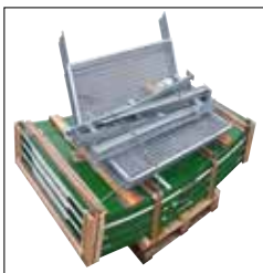
Four-part tennis wall with ball guard, packed for shipment
